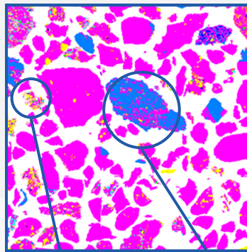
Pre-HPSA +100 mesh sample showing interspersal and association of gangue
